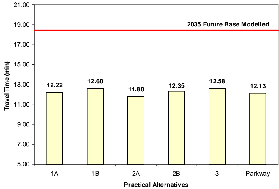
EXHIBIT 40. TRAVEL TIME COMPARISON: EASTBOUND/SOUTHBOUND PM PEAK HOUR, HOWARD AVENUE TO COLLEGE AVENUE (LOCAL TRAFFIC)
