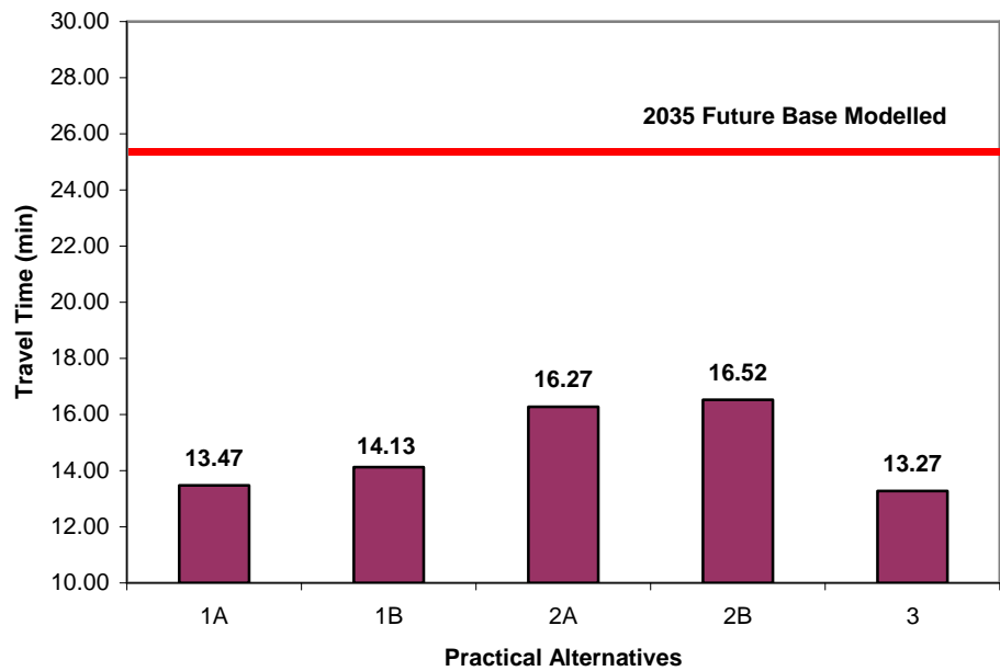
EXHIBIT 32. TRAVEL TIME COMPARISON: SOUTHBOUND/EASTBOUND PM PEAK HOUR, COLLEGE AVENUE TO HOWARD AVENUE (LOCAL TRAFFIC)
