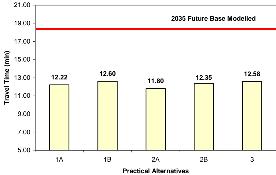
EXHIBIT 32. TRAVEL TIME COMPARISON: SOUTHBOUND/EASTBOUND PM PEAK HOUR, COLLEGE AVENUE TO HOWARD AVENUE (LOCAL TRAFFIC)
